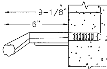
POLYPROPYLENE STEP, LANE NO. P-13938 OR EQUAL
